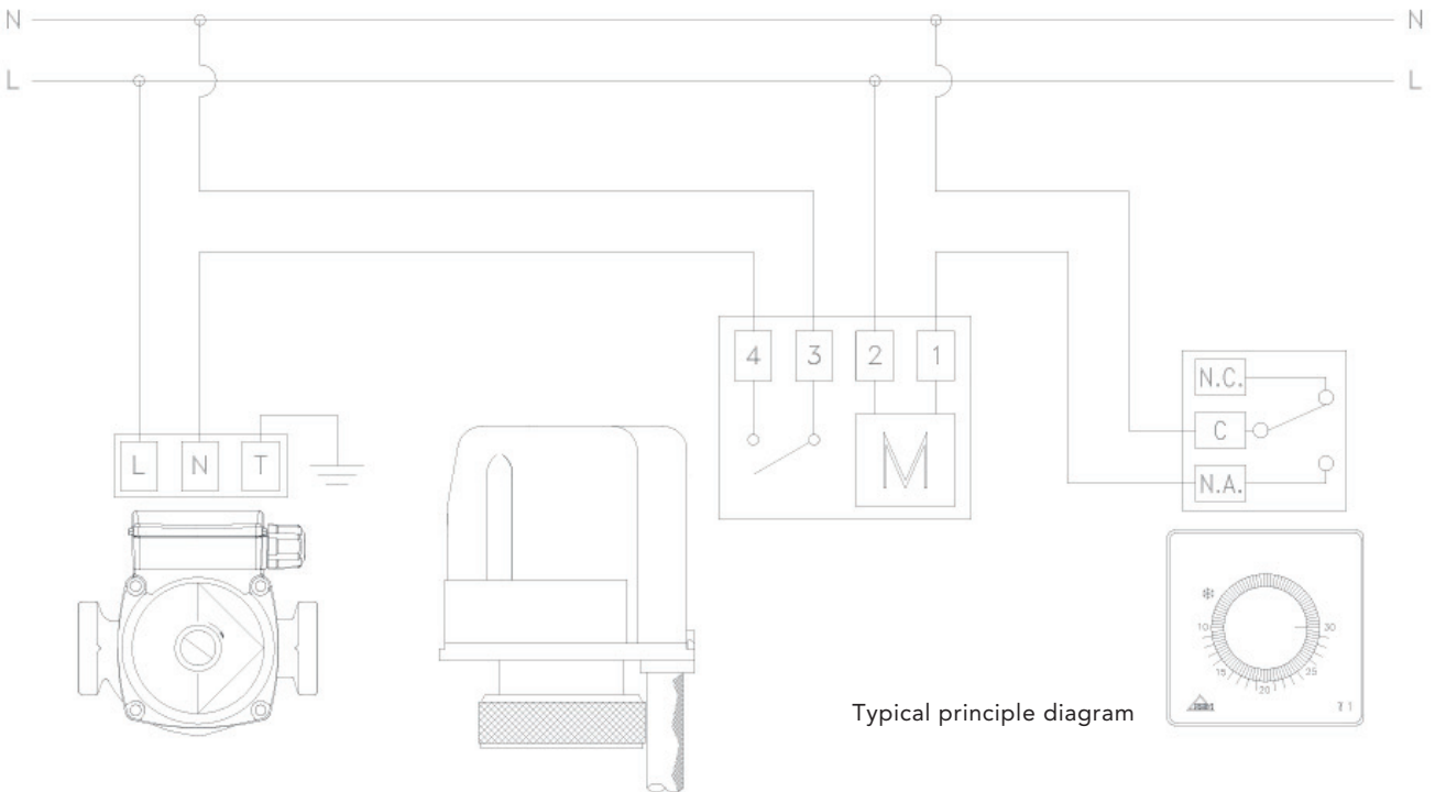
Fig.2 Electrical wiring of electrothermal actuator, equipped with auxiliary micro switch.
