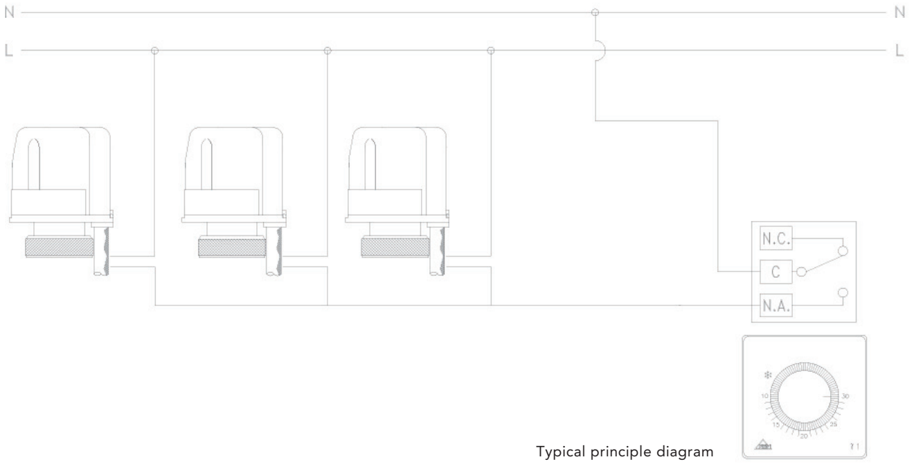
Fig.1 Electrical wiring of several electrothermal actuators, without auxiliary micro switch, installed in parallel.
